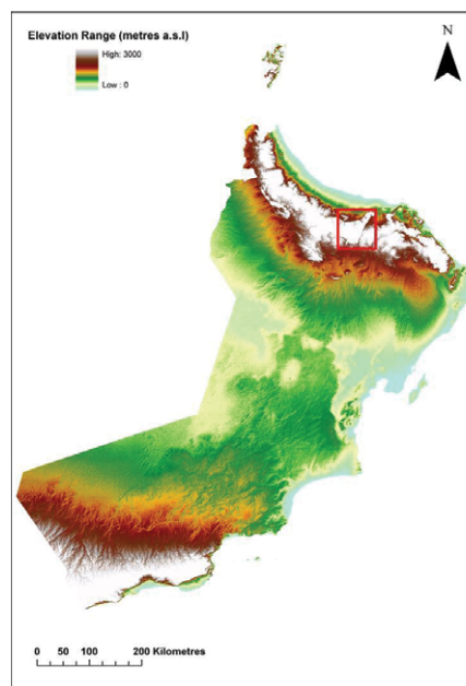
Figure 1: Digital elevation map of the Sultanate of Oman [45]. The Al Jabal Al Akhdar study area is shown in red.
