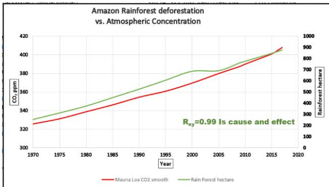
Graph 4: Rain forest deforestation vs. Atmospheric CO 2 rise (D. White 2020).
