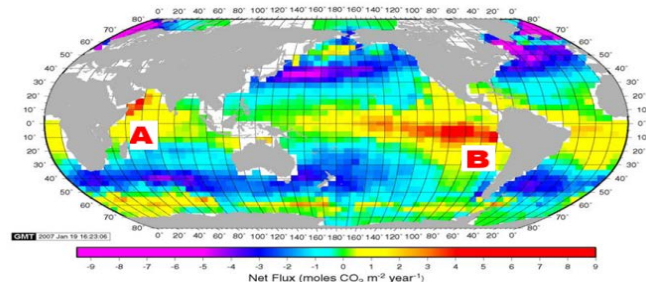
Figure 6: Takahashi 1997 Ocean Surface CO 2 [21].
