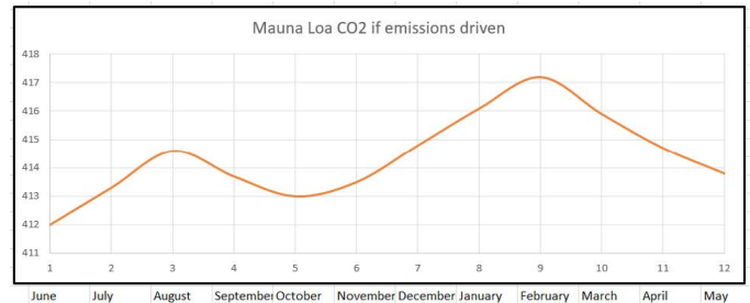
Graph 8: Mauna Loa CO 2 if emissions driven (calculated) (D. White 2020).
