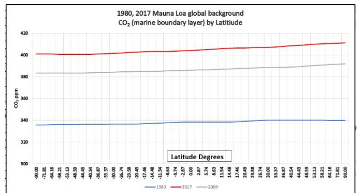
Graph 7: CO 2 mixed by atmospheric winds. (D. White, P. Tans (NOAA) 2017).
