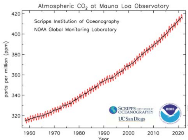
Figure 7: Mauna Loa CO 2 rise since 1960. (9/24/2021).
