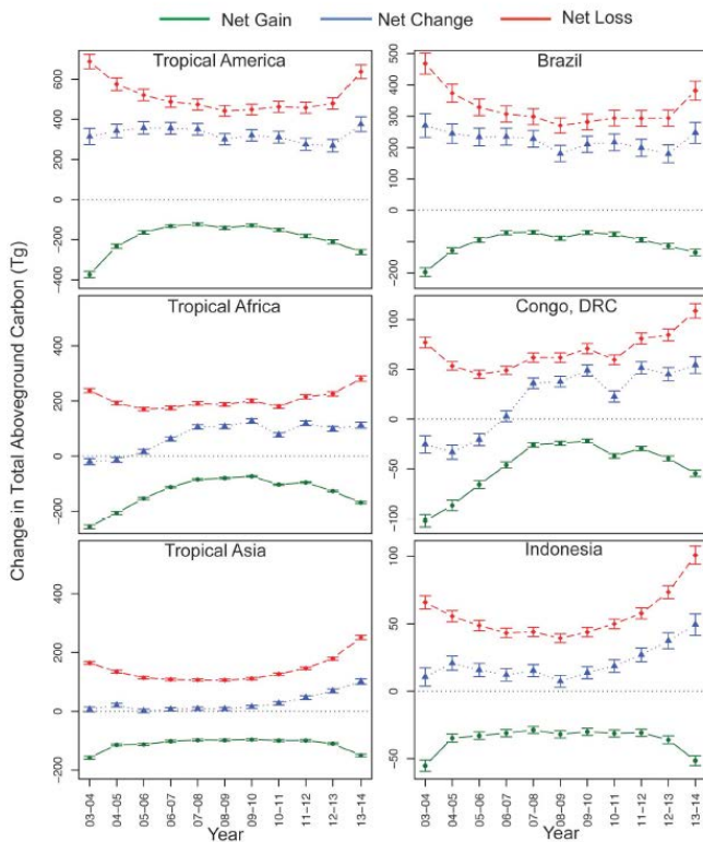
Figure 1: Figure 1: Most southern hemisphere tropical forests have switched to be an oxygen sink and carbon dioxide producer. Annual net change (95% confidence interval) in total carbon. Red lines indicate a loss in carbon; green lines indicate a gain. Blue lines reflect the difference between losses and gains. The vertical bars indicate the standard error of the change value [11].
