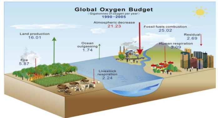
Figure 3: Worldwide Oxygen Budget [13].
