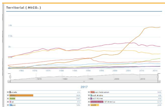
Figure 5: Global Carbon Emissions [18].
