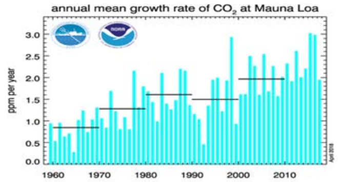
Graph 6: Mauna Loa CO 2 Rate of Rise [16].
