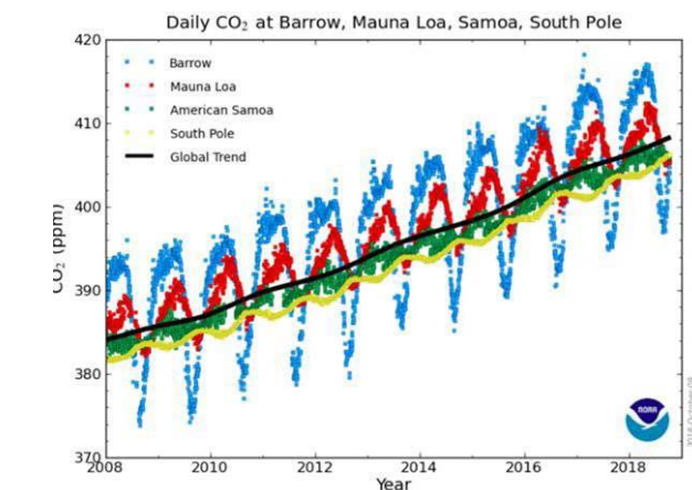
Graph 5: Mauna Loa cycles [16].
