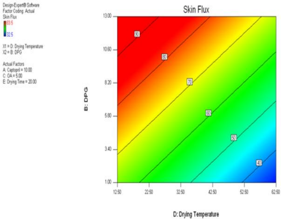
Figure 4. Response surface of Effect Analysis for skin flux
