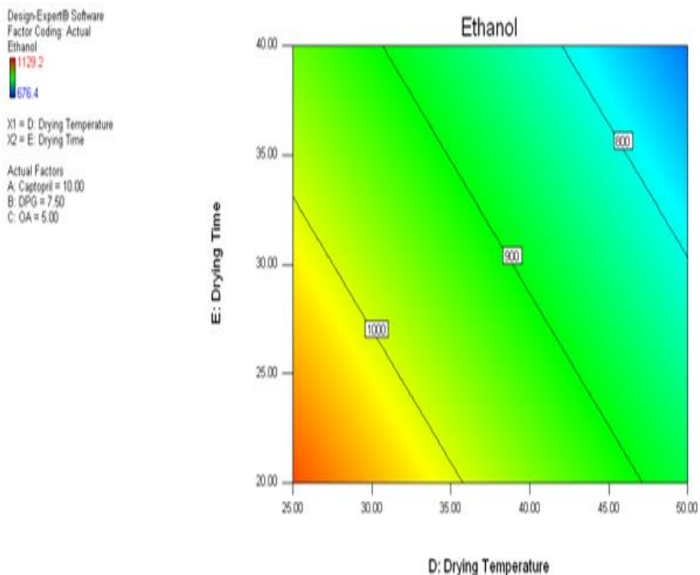
Figure 12: Response surface of Effect Analysis for ethanol
