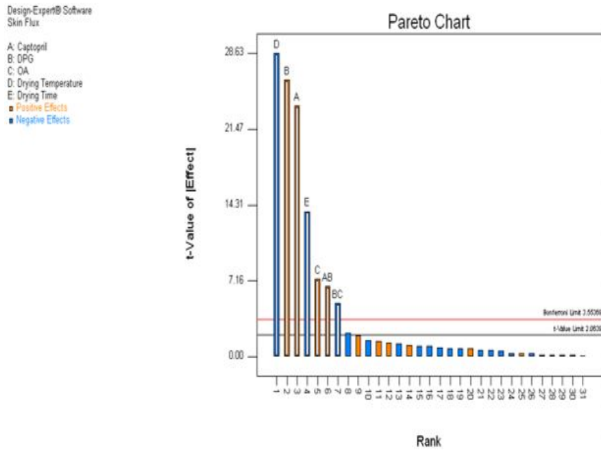
Figure 3. Pareto Chart of Effect Analysis for skin flux
