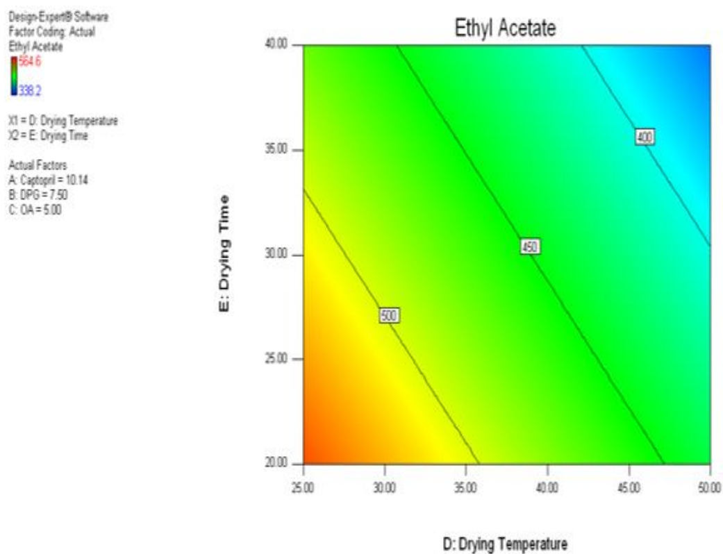
Figure 14: Response surface of Effect Analysis for ethyl acetate
