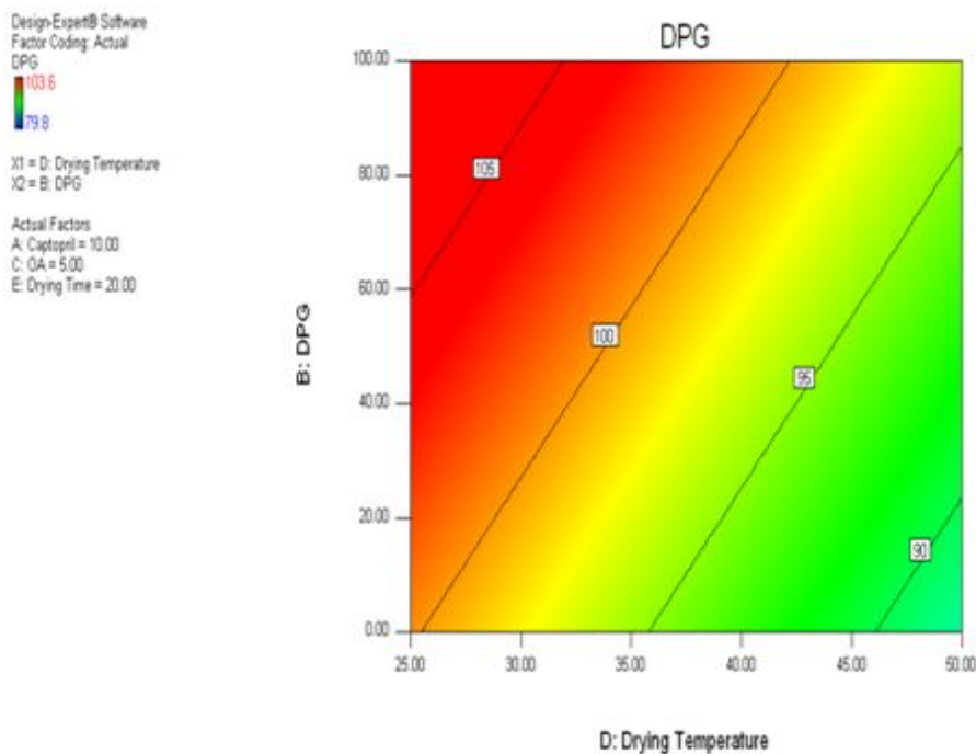
Figure 2: Response surface of Effect on DPG
