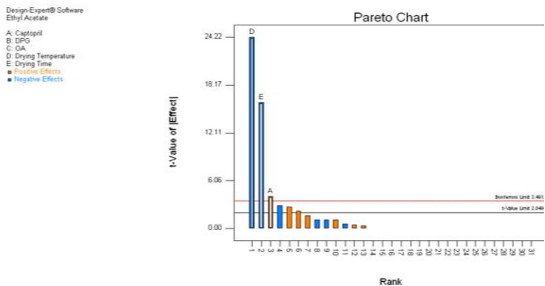
Figure 13: Pareto Chart of Effect Analysis for ethyl acetate
