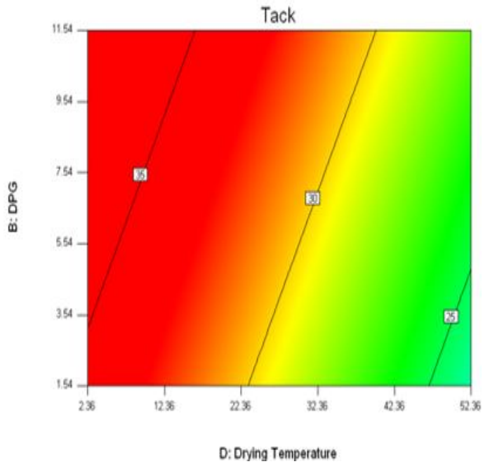
Figure 8: Response surface of Effect Analysis for Tack
