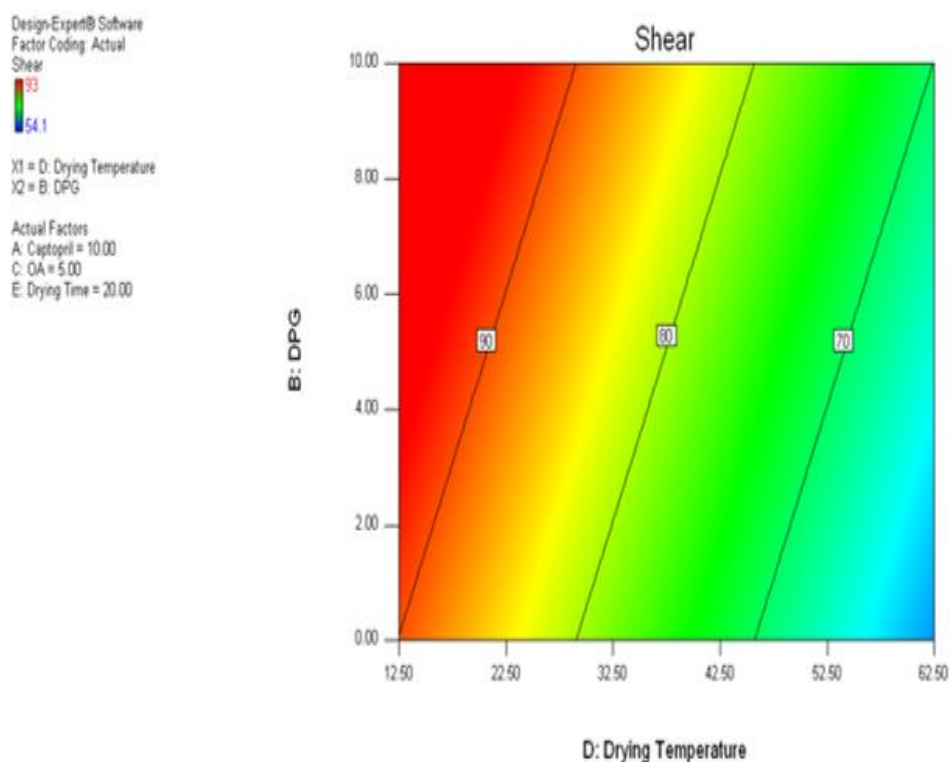
Figure 10: Response surface of Effect Analysis for shear
