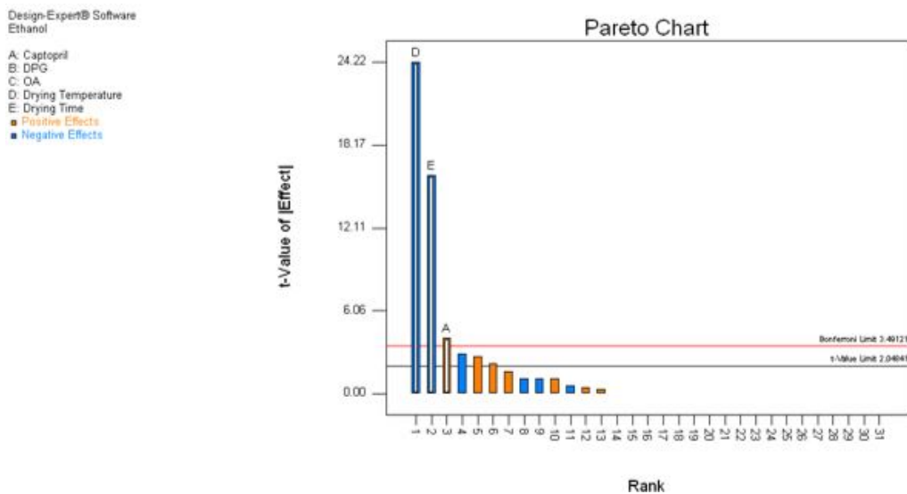
Figure 11: Pareto Chart of Effect Analysis for ethanol
