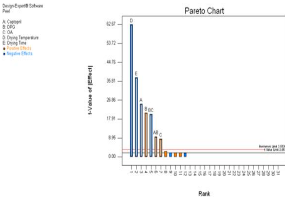
Figure 5: Pareto Chart of Effect Analysis for peel
