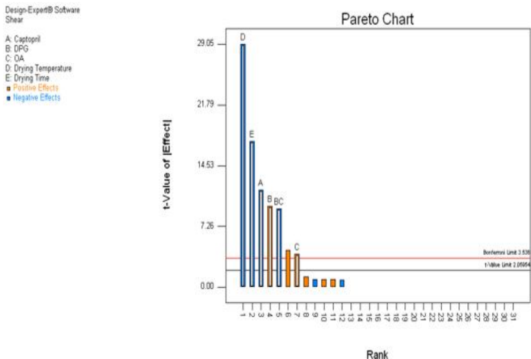
Figure 9: Pareto Chart of Effect Analysis for shear
