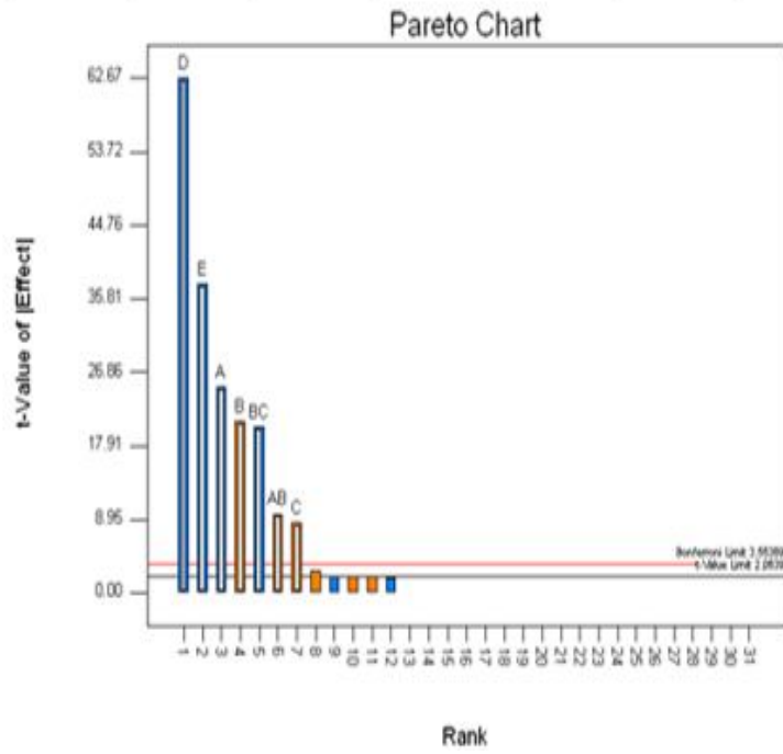
Figure 7: Pareto Chart of Effect Analysis for Tack
