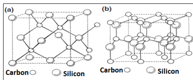
Figure 1: Crystal structures: (a) Zinc blend structure of 3C-SiC and (b) Wurtzite structure of 6H-SiC.
