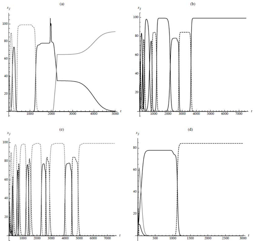
Figure 5: With variable toxin production, typical simulations indicated that one species survives (dominates) and the remaining become extinct. (a) x2 dominates. (b) x1 dominates. (c) x4 dominates. (d) x3 dominates.
