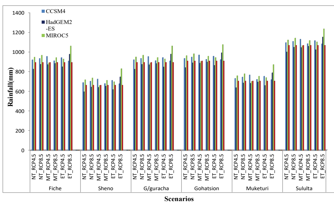
Figure 2: Future rainfall distribution of different districts in Salale zone, Oromia region.
