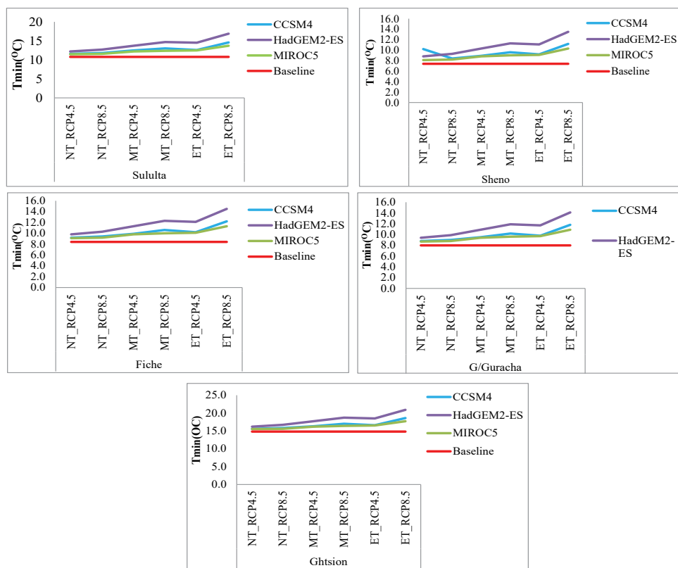
Figure 4: Future minimum temperature of meteorology stations in Salale zone, Oromia region.
