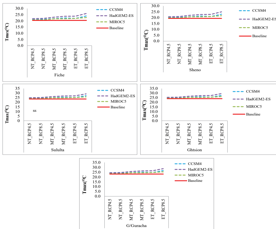
Figure 3: Future Maximum temperature of meteorology stations in Salale zone, Oromia region.
