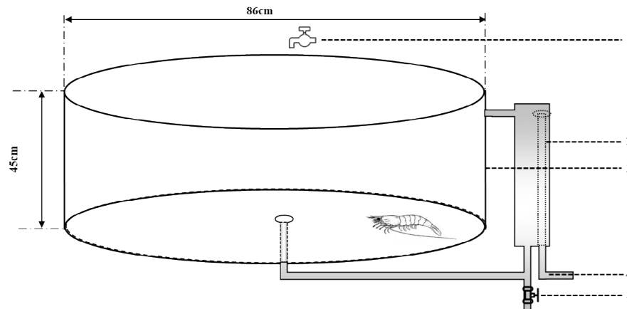
Figure 1: The drawing of small culture tanks for P. vannamei . 1- Inlet valve; 2- PVC inner tube; 3- Culture tanks; 4- Outlet piping; 5- Outlet valve.
